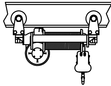
IDLER TROLLEYS MONORAIL
