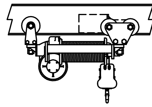
DRIVE TROLLEY MONORAIL
