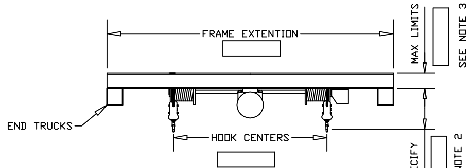
END TRUCKS BOTTOM MOUNTED HOIST
