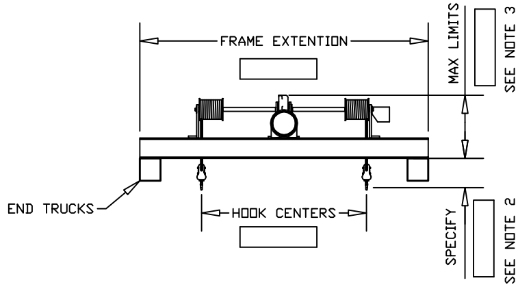
END TRUCKS TOP MOUNTED HOIST
