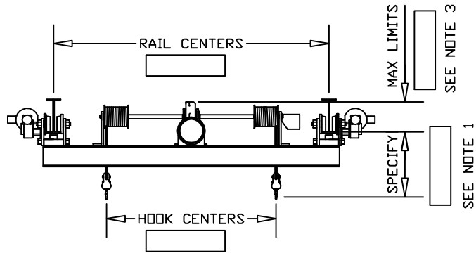
UNDERHUNG TROLLEYS TOP MOUNTED HOIST
