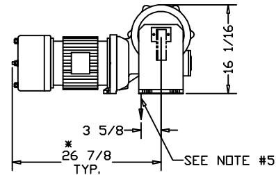
HOIST MOUNTING DETAIL HOLE LOCATIONS
